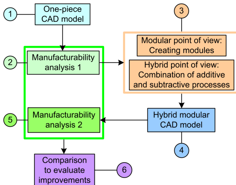
Fig. 5. Hybrid modular design methodology.
